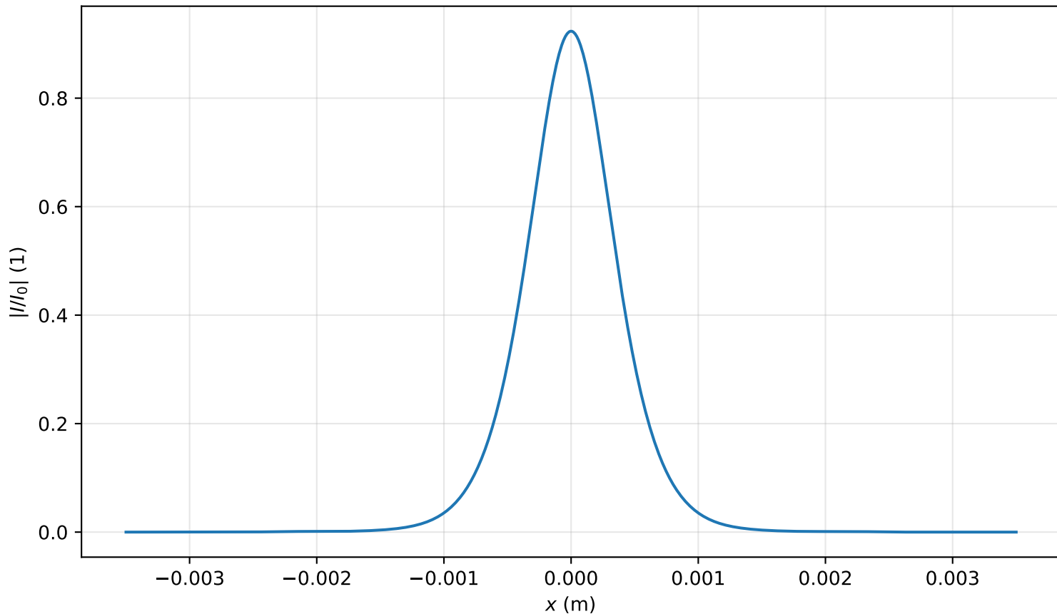
Intensity profile I(x, y = 0, z = 3.742m)/I_0 , P_{in}=0.8P_{cr} , artificial time
